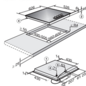
KM 3010 G (installation drawing) 1. Front, 2. Casing depth, 3. Mains connection box with mains connection cable L = 2000 mm, 4. Gas connection R 1/2" - ISO 7-1 (DIN EN 10226)
