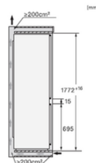
KFN7734D, KFN7734C, KFN7734F, KFN7734D, KFN7764D, KFN7785D, KFN7744E, KFN7774B, side view (installation drawings)
