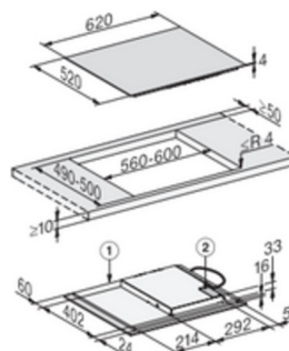
KM7360FL, KM7361FL surface-mounted (*Fußnote) (installation drawing)
