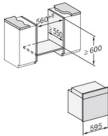
Installation H7000 XL underframe, installation drawings If the oven is to be installed under a hob, follow the instructions for installing the hob and the height of the hob.
