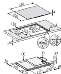
KM7360FL, KM7361FL flush (*Fußnote) (installation drawing)
