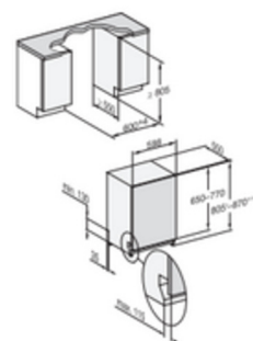
G7000, fully integrated dishwasher, 60cm (installation drawing)
