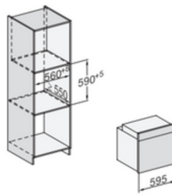
built-in H7000 XL, installation drawing
