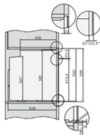
side view H7000 XL, installation drawings
