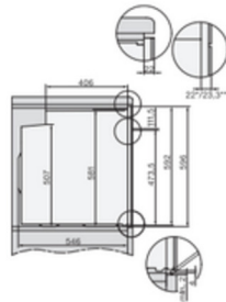
side view H7000 XL build-under, installation drawing
